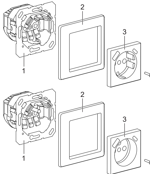
Fig. 1: Structure of the device
